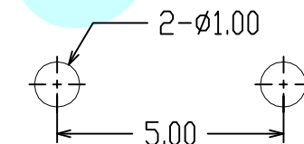
PCB Layout (Pattern Side)
