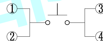
Circuit Diagram
