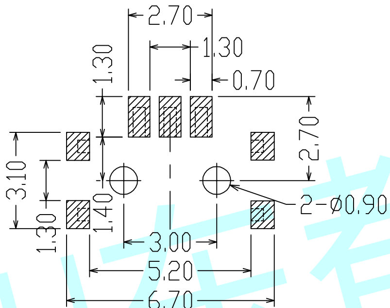
PCB Layout (Pattern Side)
