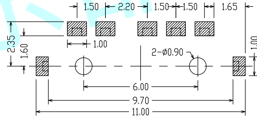
PCB Layout
