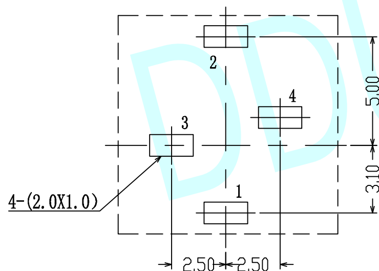
PCB Layout (Copper-Sided View)
