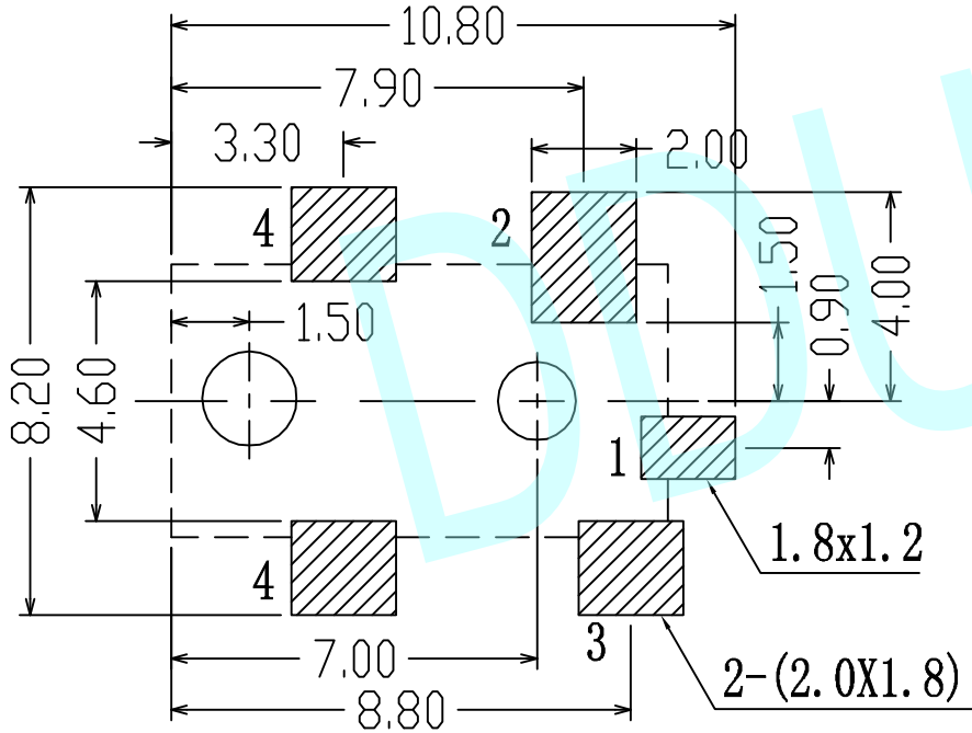
PCB Layout (Copper-Side View)
