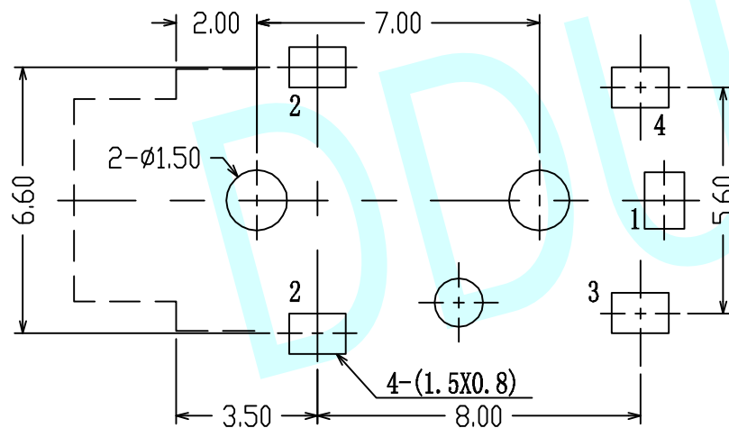
PCB Layout (Copper-Sided View)
