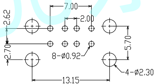
PCB Layout
