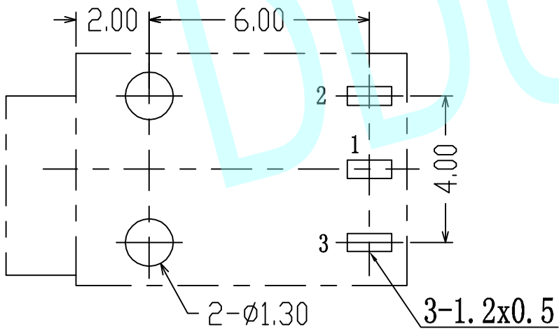
PCB LAYOUT (Copper-side view)
