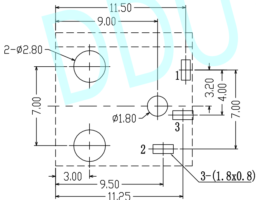
PCB Layout (Copper-Side View)
