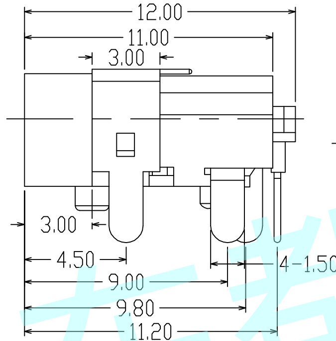
DC MATE PLUG
