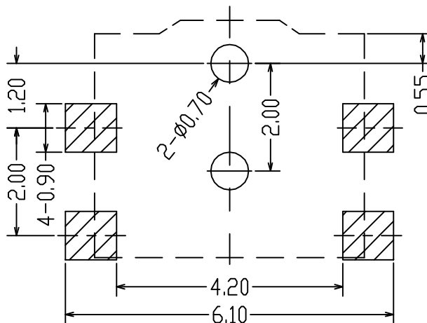
Recommended PWB Piercing Plan (Pitch Tolerance \pm 0.05 )
