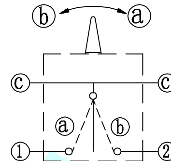
Circuit Diagram
