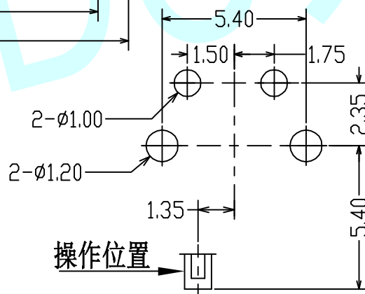
PCB Layout (Pattern Side) Scale :1:2
