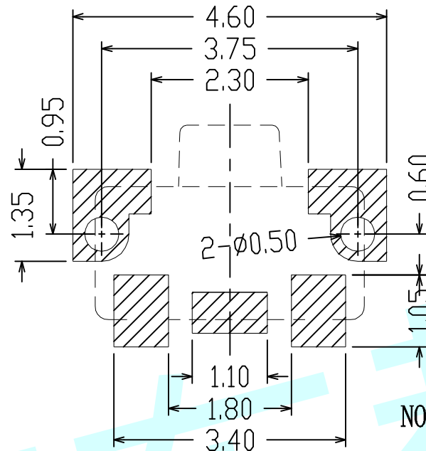
PCB Layout (Pattern Side)
