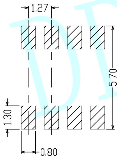
PCB Layout
